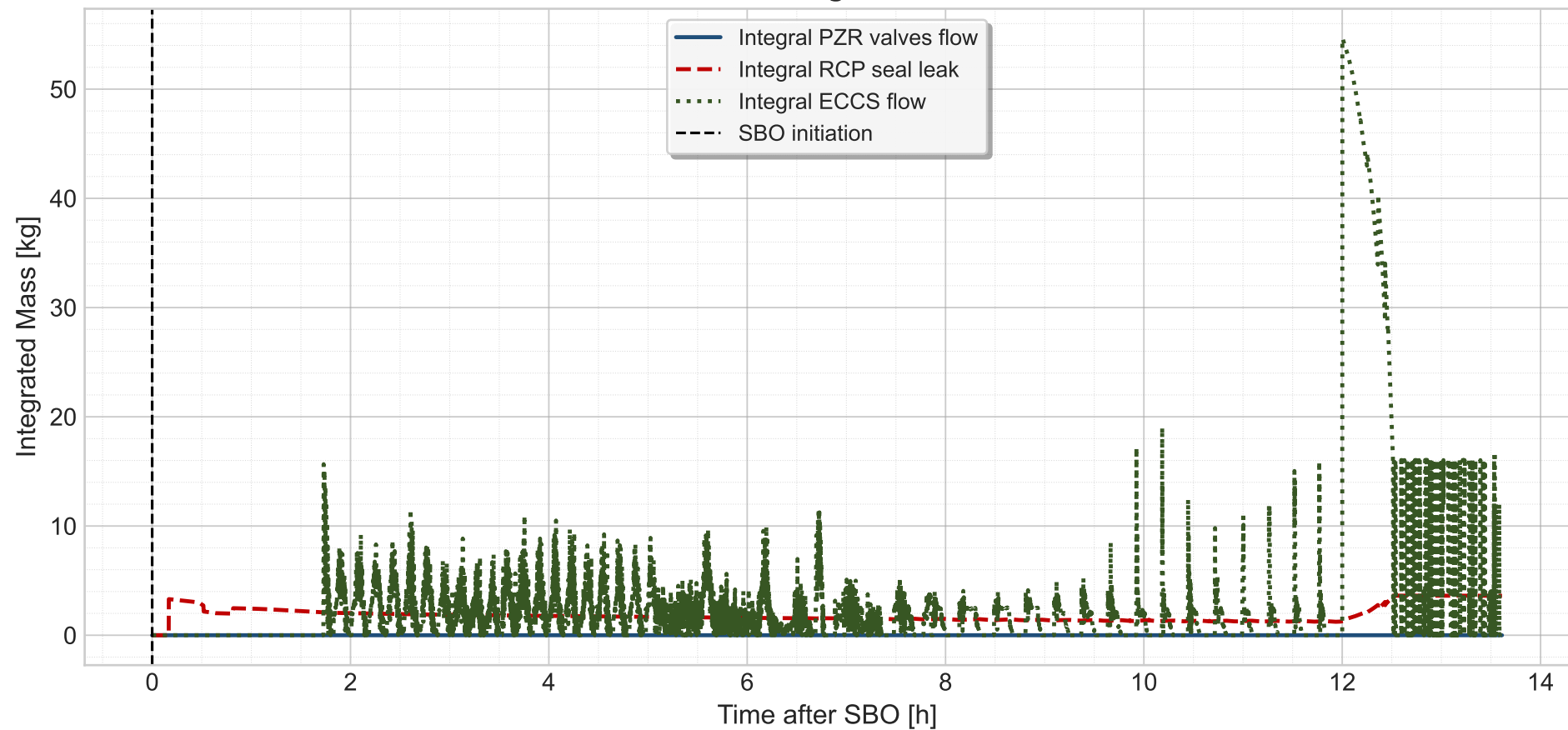
Base Case - Integral Mass Flows
